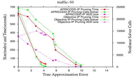
Figure 7: Detailed comparison between APRICODD-IP pruning and Objective-IP pruning for the traffic problem with 10 variables. True Approximation Error is \max_{\vec{x}} |V^*(\vec{x}) - V_{\text{approx}}(\vec{x})| .
